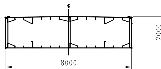
NORMAL FRAME (spacing 600mm)
