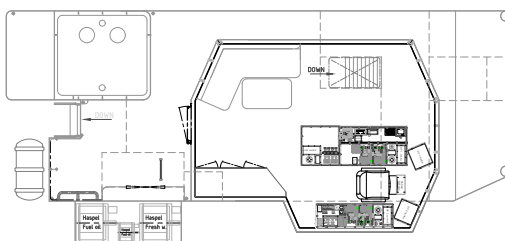
TOPVIEW ON SUPERSTRUCTUREDECK
